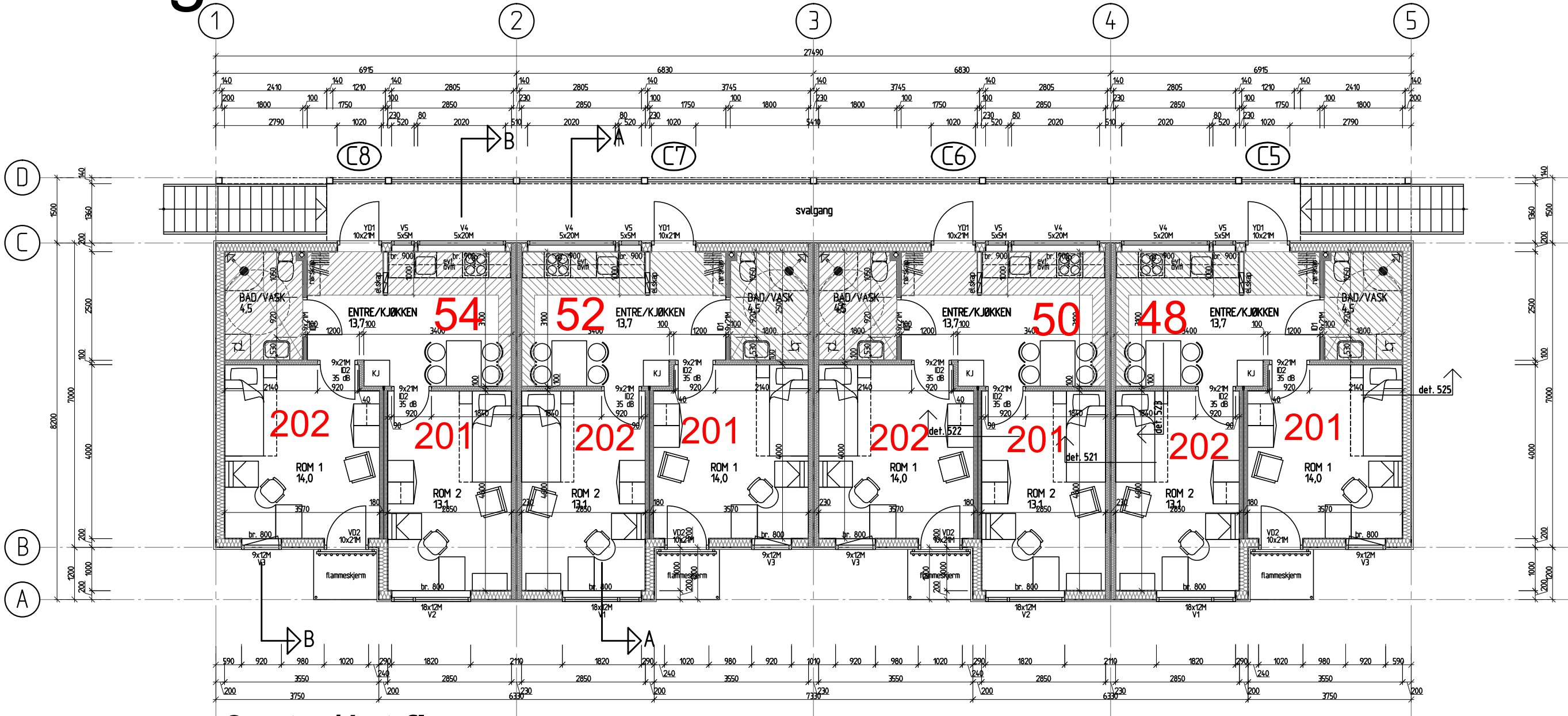
2. etg./1st floor
