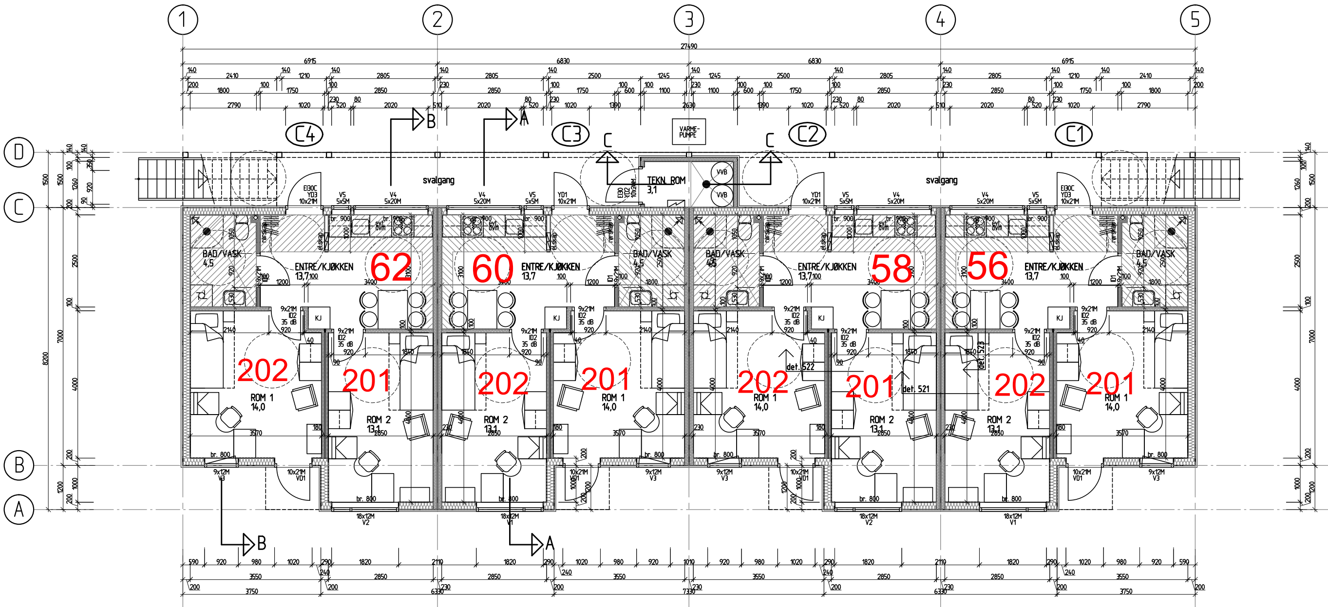
1.etg/ground floor
