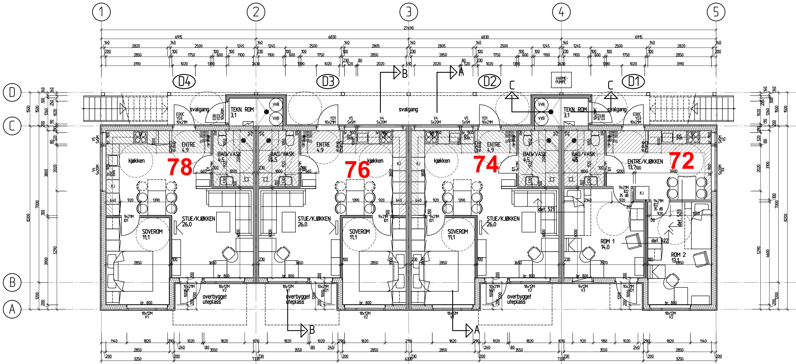
1.etg/ground floor
