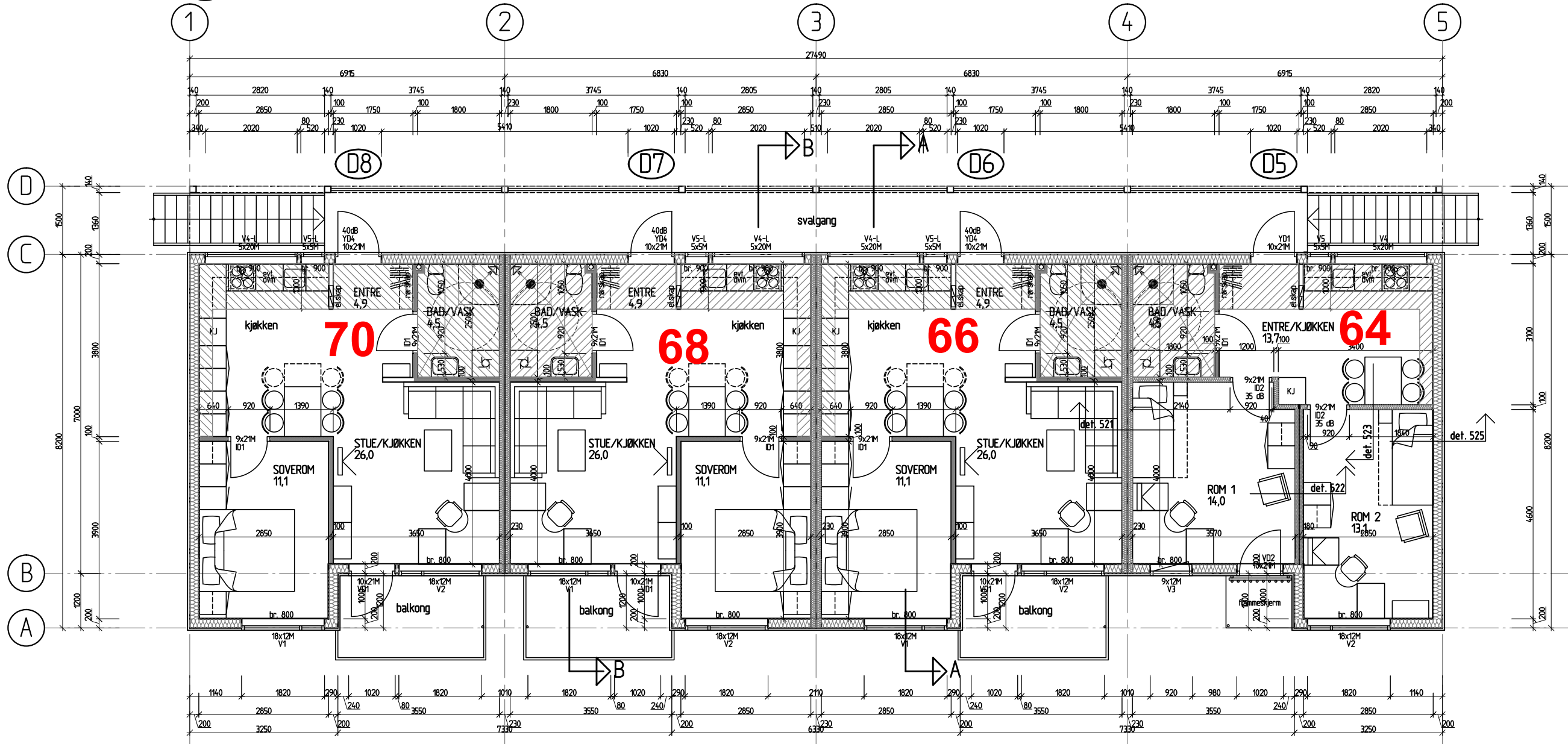
2. etg./1st floor
