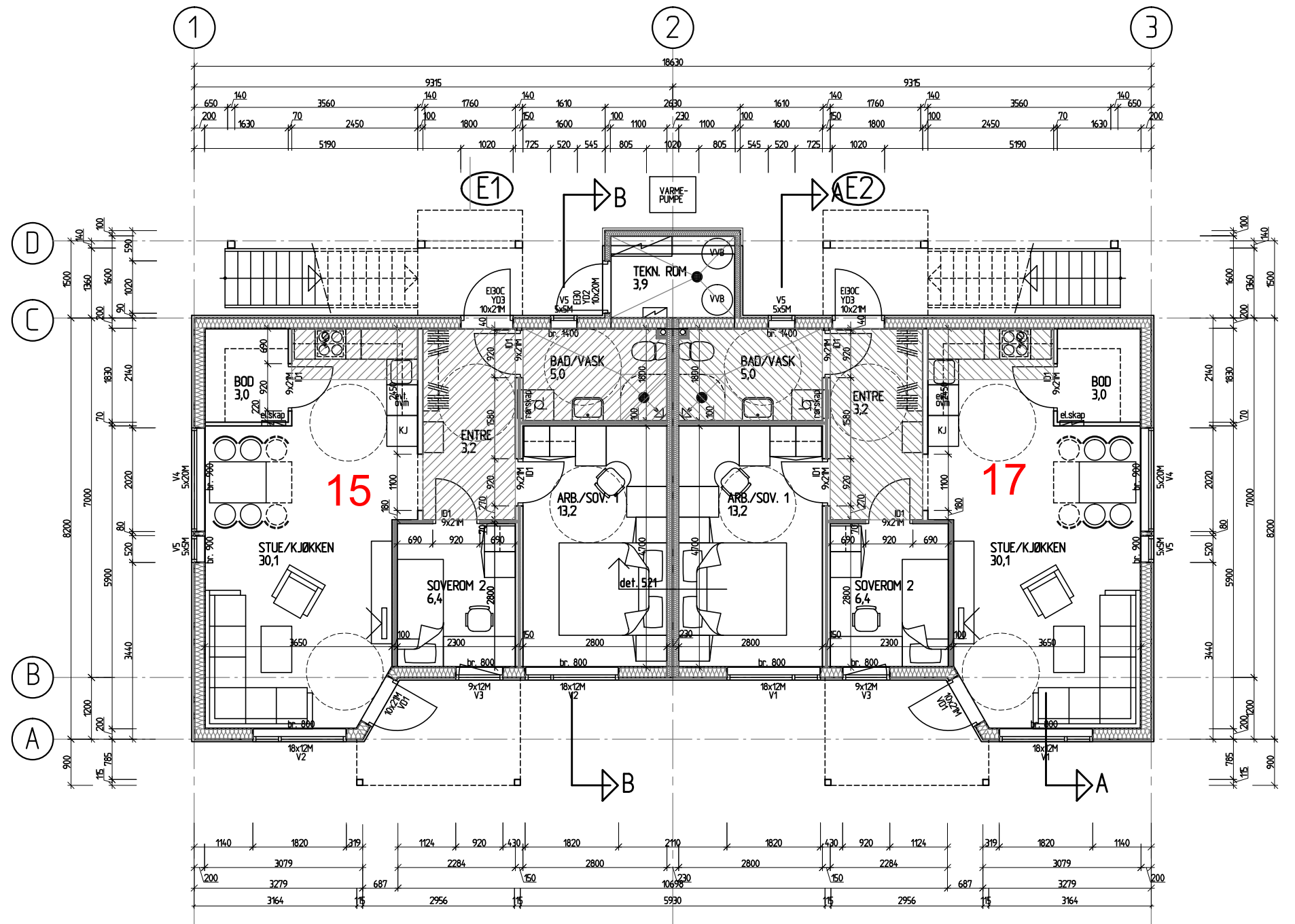
1.etg./ground floor
