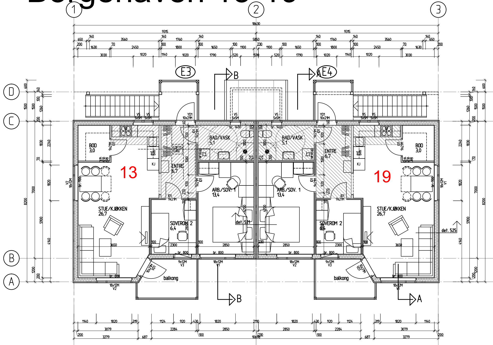
2. etg./1st floor
